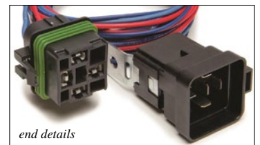
end details
