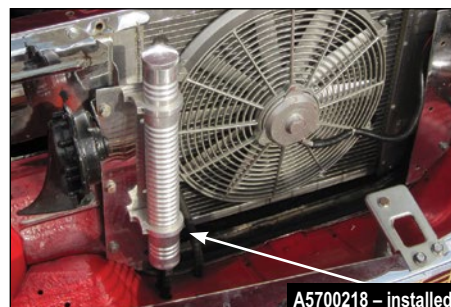
A5700218 - installed
