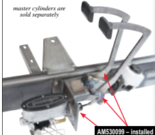
AMS50099 - installed
